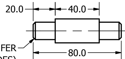
AXLE SCALE 1 / 2
