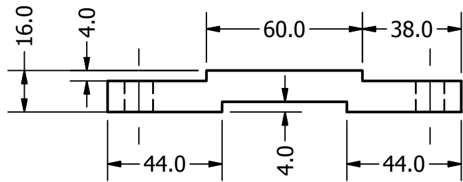
TOP PLATE SCALE 1 / 2
