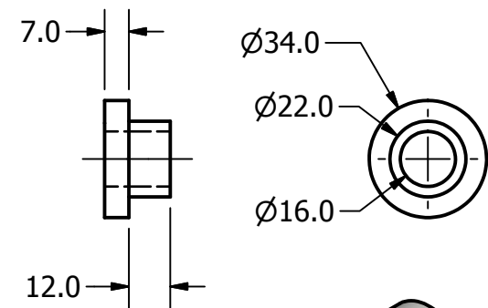
BUSHING SCALE 1 / 2
