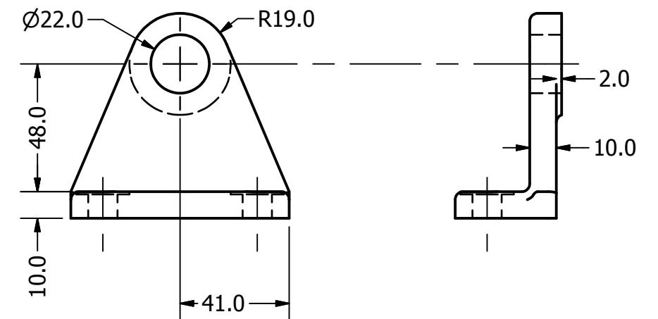
AXLE SUPPORT SCALE 1 / 2
